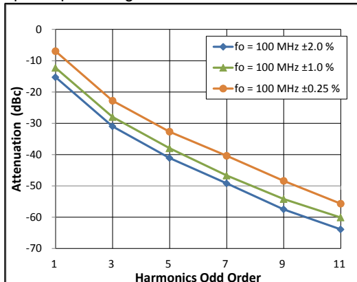
Spread percentage
