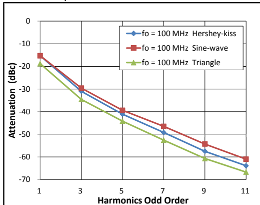
Modulation profile
