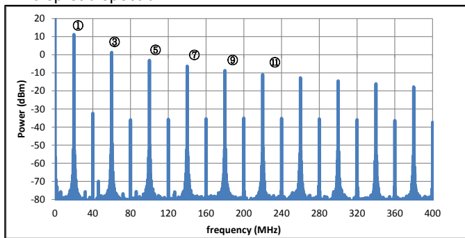
Modulation profile
